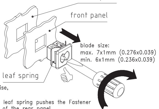
b) Installation and Removal rear panel
