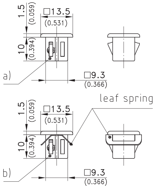
a) Installation and Removal
