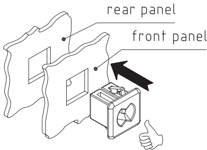
a) Installation and Removal
